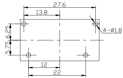
(Bottom terminals)
