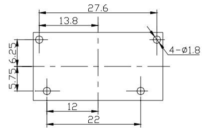
(Terminal arrangement)
