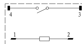
(Terminal arrangement)
